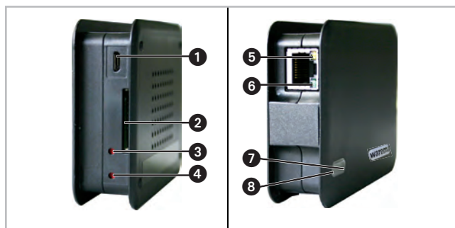
Abb. 17 Anschlüsse WebControl
